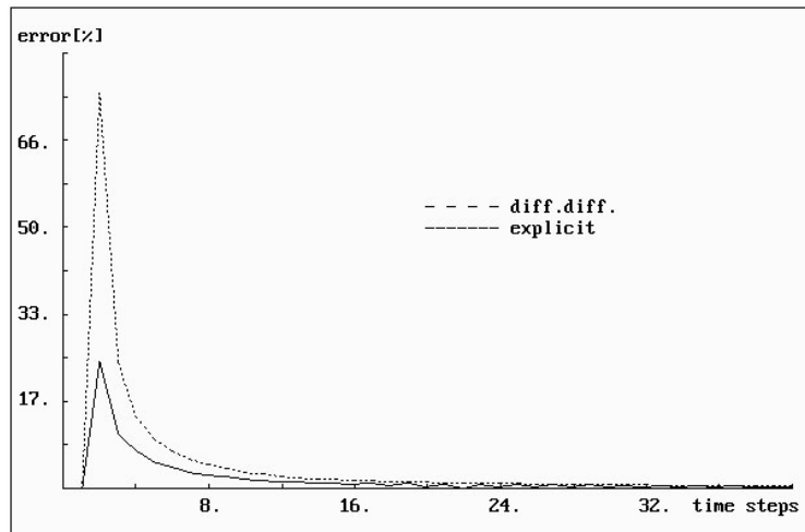
Figure 8. Comparison of the explicit and differential-difference methods in a one-layer slab where L = 0.15 m and RC = 14.3 1/h. The figure illustrates percentage errors in each case of figure 7.
