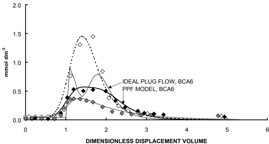
Figure 8. Theoretical and experimental breakthrough of calcium species from pulp beds (6% consistency) displaced with 1 \text{ mmol dm}^{-3} solutions of EDTA (grey symbols and curve) and BCA6 (black symbols and curve) chelants as well as by 1.5 \text{ mmol dm}^{-3} nitric acid (open symbols, dotted curve). The thin solid line represents the output of the mobile phase model without the PPF model (modeling of BCA6 experiment). The fiber properties and the metal amounts are those given in Table 2, Papers III–IV. Model calculations were carried out by assuming 10 CSTR units in series, 1000 channels and Pe = 50 in the PPF model. For further details of the experiment and model calculation, see Papers III–IV.
