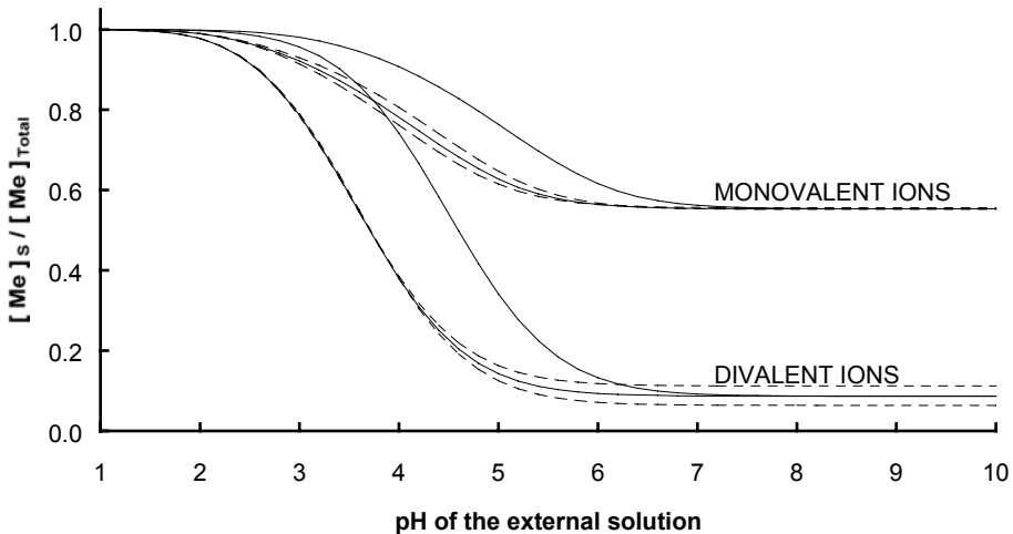
Figure 9. The theoretical concentrations of monovalent and divalent ions in external solution of 5% pulp suspension as a function of varying dissociation constant ( -\log K ) of single fiber-bound group in range 3–4 (solid lines) and FSP of fibers in range 1–2 \text{dm}^3 \text{kg}^{-1} (dotted lines). Solid lines were calculated using \text{FSP} = 1.5 \text{ dm}^3 \text{ kg}^{-1} . The metal amounts used in the calculation were those given in Table 2, Paper II. No chelant was assumed to be present in suspension. The concentration curves shift on the right with an increasing dissociation constant and reach a lower concentration level with increasing FSP, which can only be seen in curves of the divalent ion in this modeling example.
