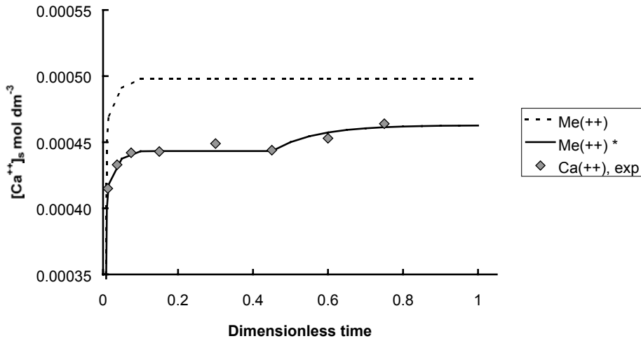
Figure 6. Ion exchange kinetics in 1% thermomechanical pulp – water suspension in presence of calcium ions and calcium carbonate. The dimensionless time T = 1 is equal to 400 minutes. Kinetic rate constants normalized to dimensionless time scale are K_\lambda = 0.97 and K_j = 0.1 , which indicate that the ion exchange between phases occur almost instantaneously and that the rate of secondary kinetics is lower by order of magnitude. The dotted line represents a modeling result without assumption of secondary kinetics.
