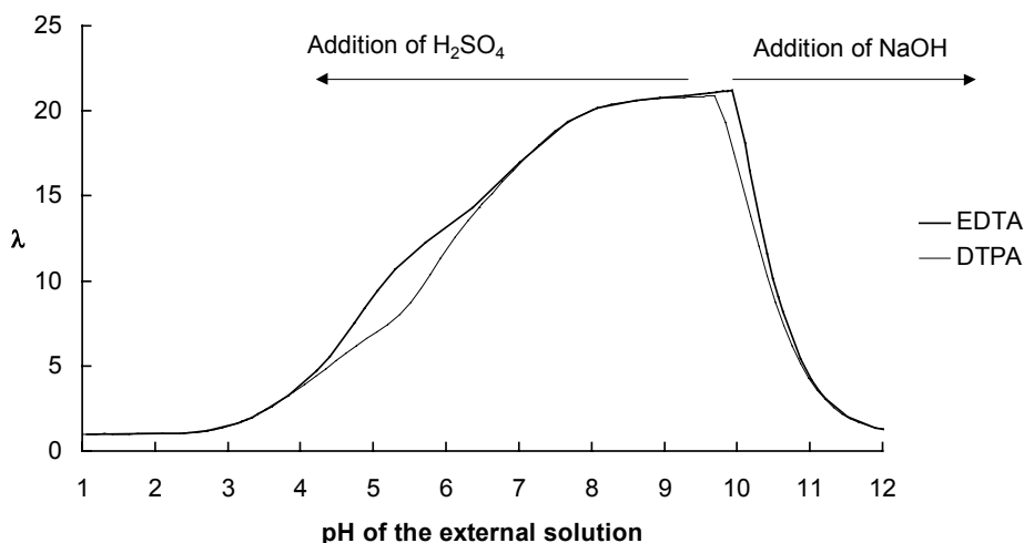
Figure 4. The calculated Donnan distribution coefficient as a value of pH in fiber suspension with EDTA and DTPA. The fiber properties and the metal amounts used in the calculation have been given in Table 2 for Paper II. The consistency of fiber suspension was 4.8% and the calculated doses of chelants were 0.0153 \text{ mol kg}^{-1} o.d. fibers in both experiments. See Paper II for further details of experiments.
