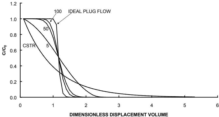
Figure 7. Theoretical removal of non-ionic substance (e.g. methanol or glucose) from a pulp bed (6% consistency) shown as a function of dimensionless displacement volume and displacement efficiency. The numbers shown denote Peclet numbers used in the modeling. The curve denoted as “Ideal Plug Flow” is the output of a mobile phase model consisting of 10 CSTR units in series.
