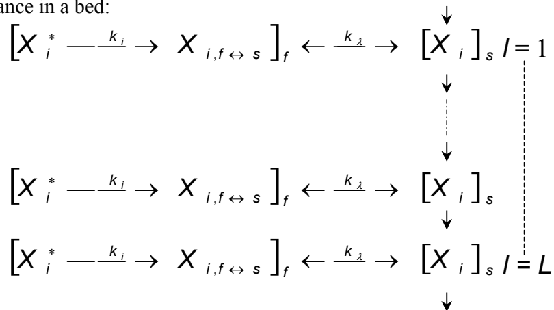
Figure 3. Extension of a kinetic ion exchange model to a mobile model and to a pulp bed model.
