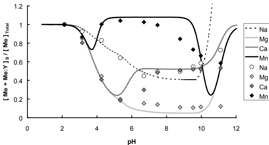
Figure 5. The experimentally determined and calculated fractions of metals in the external solution of total amount of metals present in the fiber suspension in 4.8% consistency and with calculated amount of DTPA = 0.0153 mol kg -1 o.d. fibers. See Table 2 and Paper II for the pulp properties, metal amounts and further details of the experiment.
